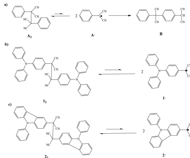
Fig. 12 (a) Equilibrium between A 2 and A * , and isomerization to B. (b) Equilibrium between I 2 and I * , (c) equilibrium between 2 2 and 2 * , reproduced from ref. 45 with permission from Wiley, Angew. Chem., Int. Ed. , 2016, 55, 8634–8638, copyright 2016.
