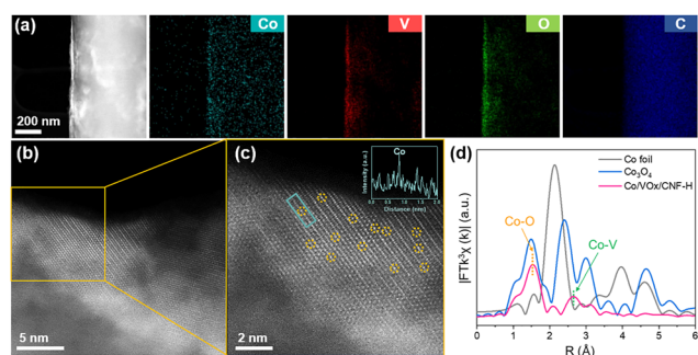
Fig. 3 (a) HAADF-STEM image of Co/VO_x/CNF-H and corresponding elemental distribution maps. (b) High-magnification HAADF-STEM image and (c) magnified image and z-contrast profile of the region highlighted in (b). (d) Fourier transformed k^3 -weighted Co K-edge of EXAFS spectra.
