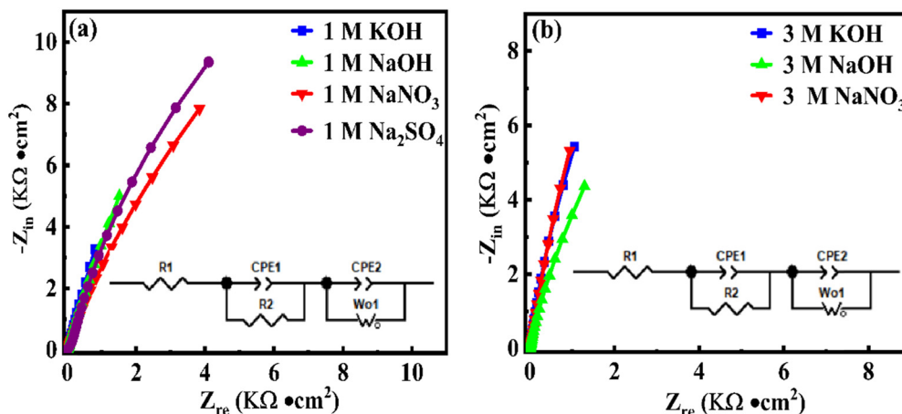
Fig. 19 Nyquist plots of Mn_2O_3-9 in (a) 1 M and (b) 3 M concentrations of different electrolytes. The insets are the equivalent circuits.
