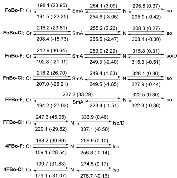
Fig. 8 Phase transition temperatures ( ^{\circ}\text{C} ) and enthalpies ( \text{kJ mol}^{-1} ) of derivatives with the inner benzoxazole (Bo) partially and fully fluorinated. Values are determined by DSC at 5^{\circ}\text{C min}^{-1} under \text{N}_2 for 2nd-heating and 1st-cooling runs. Cr = crystalline phase; SmA = smectic A; N = nematic; Iso = isotropic liquid; D = decomposition.
