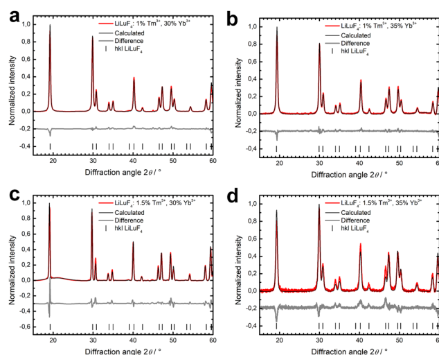
Fig. 3 Rietveld refinement of the PXRD patterns ( Cu K\alpha radiation) of the LiLuF_4:Tm^{3+}, Yb^{3+} NCs with different PXR activator ratios of Tm and Yb . LiLuF_4 (#PDF 00-027-1251). 54 (a) 1% Tm^{3+} , 30% Yb^{3+} , (b) 1% Tm^{3+} , 35% Yb^{3+} , (c) 1.5% Tm^{3+} , 30% Yb^{3+} , and (d) 1.5% Tm^{3+} , 35% Yb^{3+} .
