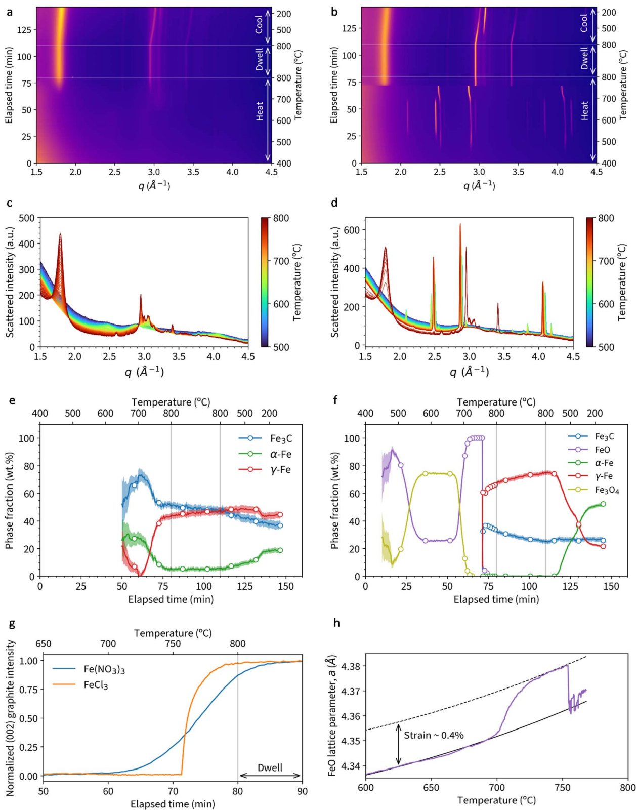
Fig. 2 Heatmaps of WAXS data for samples of (a) cellulose + \text{Fe}(\text{NO}_3)_3 and (b) cellulose + \text{FeCl}_3 heated to 800 °C under nitrogen. Also diffraction data for (c) cellulose + \text{Fe}(\text{NO}_3)_3 and (d) cellulose + \text{FeCl}_3 with an additional panel showing the temperature for each pattern during heating to 800 °C. Phase fractions extracted from Rietveld refinement of data for (e) cellulose + \text{Fe}(\text{NO}_3)_3 and (f) cellulose + \text{FeCl}_3 . A plot of (g) normalised graphite (002) peak intensity vs. time and temperature. (h) Plot showing expansion of FeO lattice parameter a with increasing temperature.
