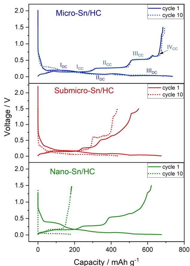
Fig. 2 Galvanostatic cycling of micro-, submicro- and nano-Sn/HC electrodes (8 : 2 wt%) cycled at 50\ \text{mA g}^{-1} (1 st cycle) and at 100\ \text{mA g}^{-1} (10 th cycle). Tests conducted at 25\ ^\circ\text{C} within the 0.01\text{--}1.5\ \text{V} range. Electrolyte: 1\ \text{M NaPF}_6 in diglyme.
