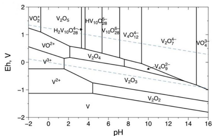
8 Fig. 2. Eh–pH diagram for vanadium species at [V]=1M^{43} (Reprinted with permission 9 of American Chemical Society)
