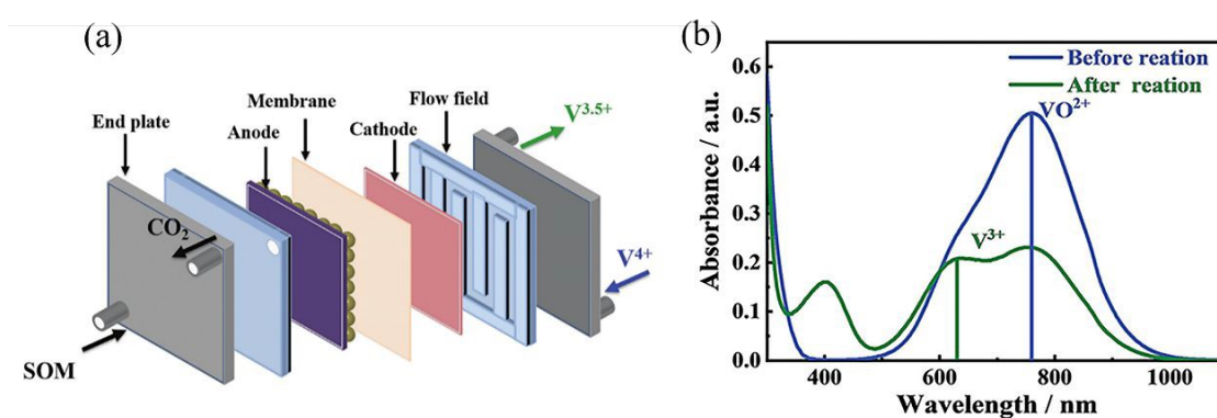
7 8 Fig. 13. (a) Schematic diagram and reaction mechanism of fuel cell reactor; (b) UV- 9 vis spectra of the electrolytes before and after reaction 52 (Reprinted with permission of 10 MDPI)
