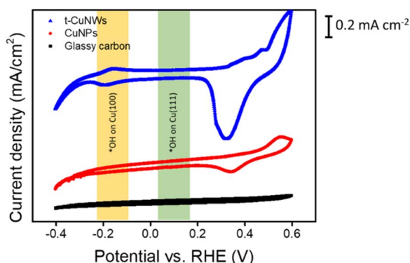
Fig. 2 Cyclic voltammetry of glassy carbon electrode, CuNPs and t-CuNWs in Ar-saturated 1 \text{ M KOH} from -0.4 to 0.6 \text{ V} vs. RHE with a scan rate of 50 \text{ mV s}^{-1} . Note that the cyclic voltammetry shown corresponded to the fifth cycle, which overlapped with the preceding four cycles as shown in Fig. S6, indicating stable electrochemical response.
