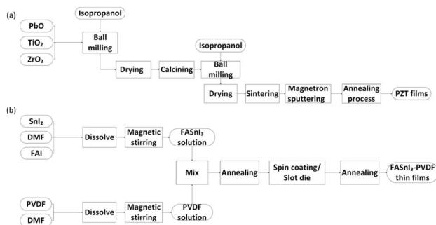
Fig. 2 Flowcharts of the manufacturing process of (a) typical PZT piezoelectric ceramic deposited in thin films by RF-magnetron sputtering and (b) FASnI 3 -PVDF perovskite deposited in thin films by spin coating/slot-die.
