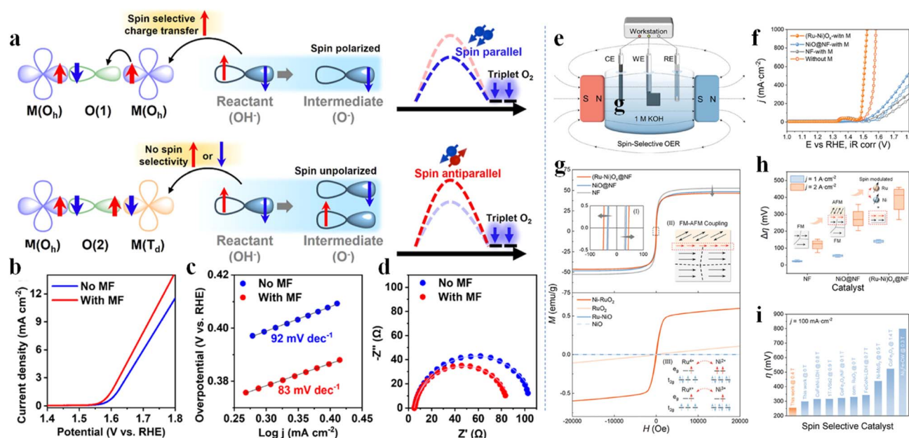
Fig. 11 (a) Mechanism of the spin-selective charge transfer of adsorbed OH - ions through the M(OH)–O(1)–M(OH) and the M(OH)–O(2)–M(Td) sites in CFO. (b) LSV curves of CFO recorded in 1 M KOH electrolyte. (c) Tafel slopes of CFO recorded in 1 M KOH electrolyte. (d) Nyquist plots of CFO recorded in 1 M KOH electrolyte with and without magnetic field applied. Reproduced with permission. 106 Copyright 2025 American Chemical Society. (e) Schematic illustration of a three-electrode system with an external magnetic field. (f) LSV curves of the (Ru–Ni)O x @NF, NiO@NF, and NF in 1.0 M KOH. (g) Magnetization hysteresis loops of the (Ru–Ni)O x @NF, NiO@NF, NF, RuO 2 , NiO, RuO 2 (Ni-1.3%), NiO (Ru-1.1%) at room temperature. (h) Changes in \eta at j = 1 and j = 2 A cm -2 of the (Ru–Ni)O x @NF, NiO@NF, and NF. (i) Comparison of \eta at j = 100 A cm -2 between the (Ru–Ni)O x @NF and the reported state-of-art spin selective OER catalysts. Reproduced with permission. 107 Copyright 2025 Wiley-VCH.
