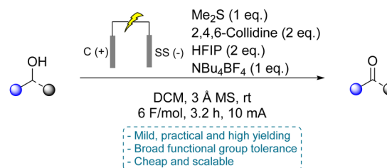
Scheme 1 Advantages and drawbacks of traditional oxidation methods compared to this work.
