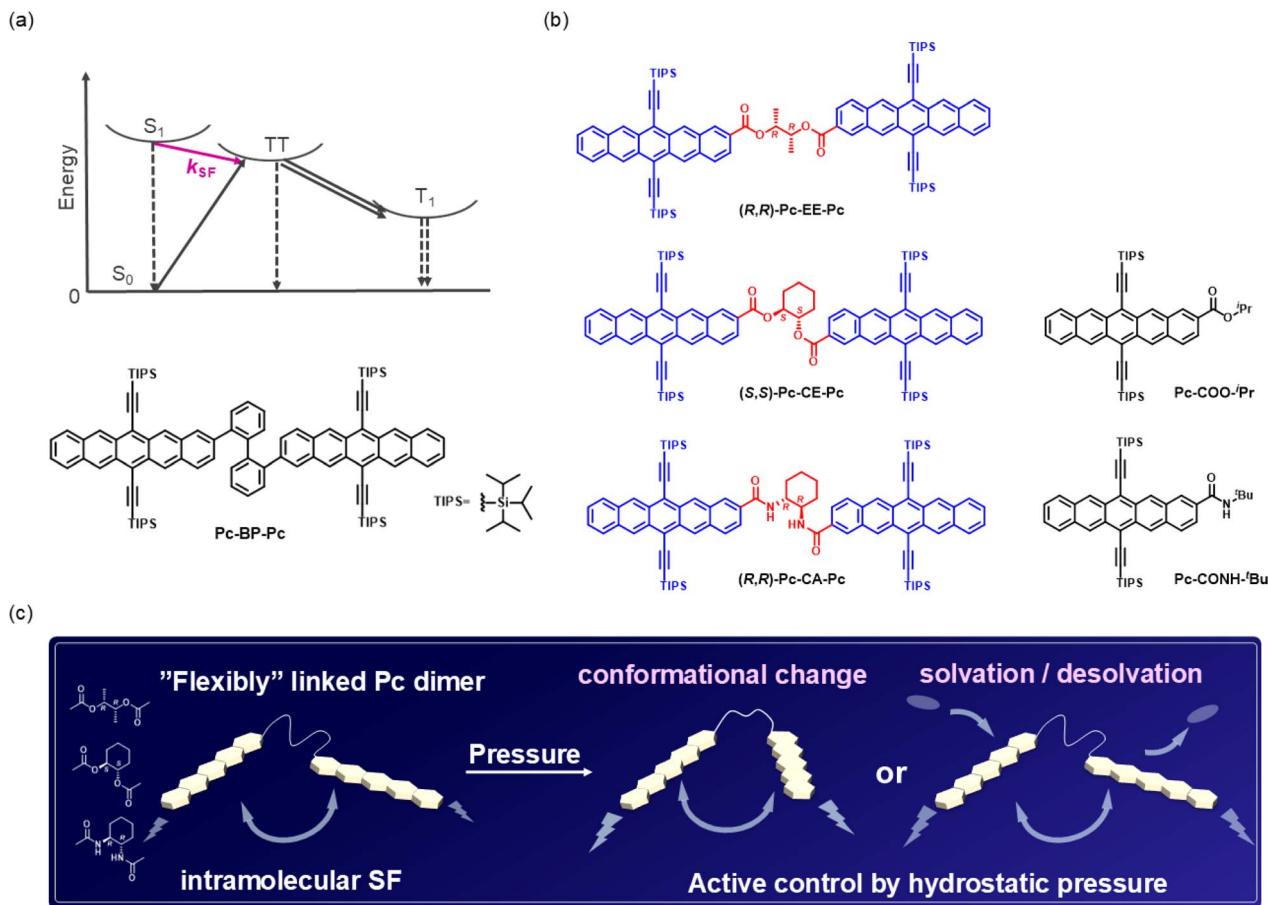
Fig. 1 (a) (Top) schematic diagram of SF in a TIPS-modified pentacene (Pc) dimer: k_{SF} represents the rate constant of SF from S_1 to TT ; in the present Pc case, the reverse triplet–triplet annihilation (TTA) can be omitted, due to the large exergonic reaction (ca. 0.3 eV). 45 (Bottom) chemical structure of Pc-BP-Pc . (b) Chemical structures of SF-active dimers; (R,R)-Pc-EE-Pc , (S,S)-Pc-CE-Pc , and (R,R)-Pc-CA-Pc , the corresponding referenced monomers; Pc-COO- i Pr and Pc-CONH- i Bu . (c) Conceptual illustration of active control of SF-active soft materials driven by hydrostatic pressure.
