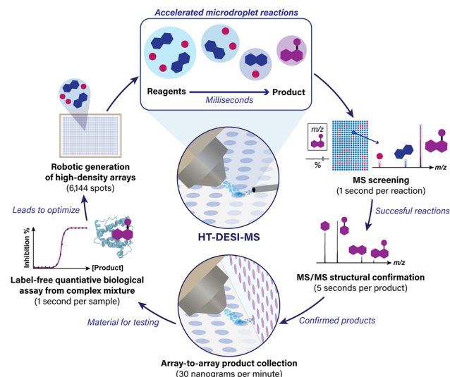
Fig. 2 Closed-loop drug discovery workflow enabled by DESI-MS and associated accelerated reactions in microdroplets.
