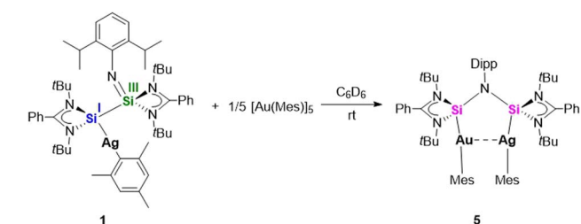
Scheme 4 Synthesis of the heterobimetallic bis-silylene complex [LSi{Ag(Mes)}–(NDipp)–{Au(Mes)}SiL] ( 5 ).
