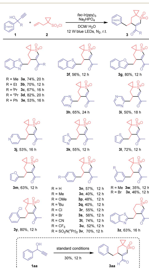
Scheme 2 Demonstration of broad functional group compatibility. Reaction conditions: 1 (0.2 mmol), 2 (0.3 mmol), Na 2 HPO 4 (0.2 mmol), and fac -Ir(ppy) 3 (3 mol%) in DCM/H 2 O (v/v 2 mL/0.2 mL), irradiated with 12 W blue LEDs at room temperature under N 2 . Yields of isolated products are given.
