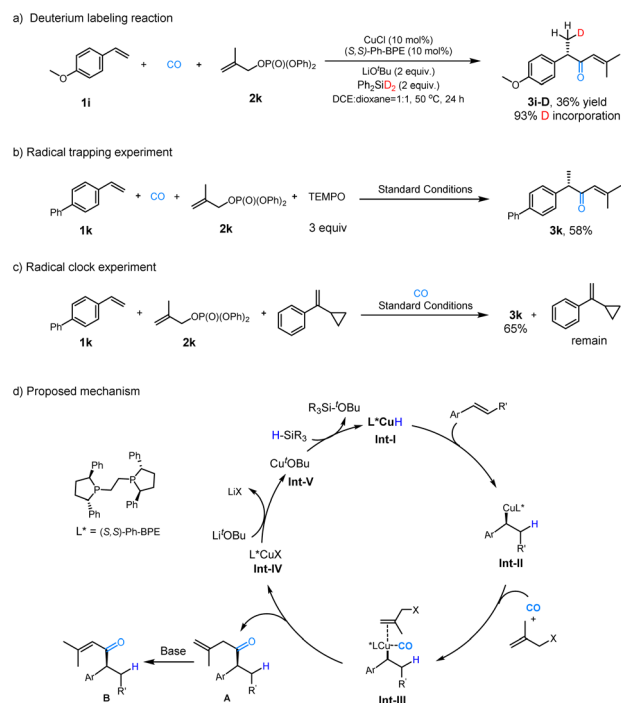
Fig. 3 Mechanism investigation experiments and proposed mechanism. Standard conditions: CuCl (10 mol%), ( S,S )-Ph-BPE (10 mol%), LiO t Bu (2.0 equiv.), (MeO) 2 MeSiH (2 equiv.) and CO (10 bar) in DCE (0.5 mL) and 1,4-dioxane (0.5 mL) at 50 °C for 24 h.
