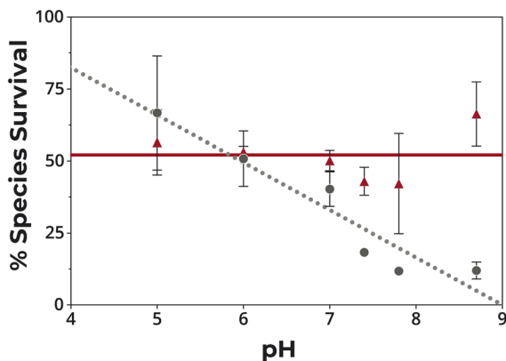
Fig. 5 Survival of GCG in the presence of UV light at different pH with and without Zn 2+ . 5 mM GCG in 20 mM GG after exposure to light at 254 nm for 16 min in the absence (gray circles) and presence (red triangles) of 5 mM Zn 2+ .
