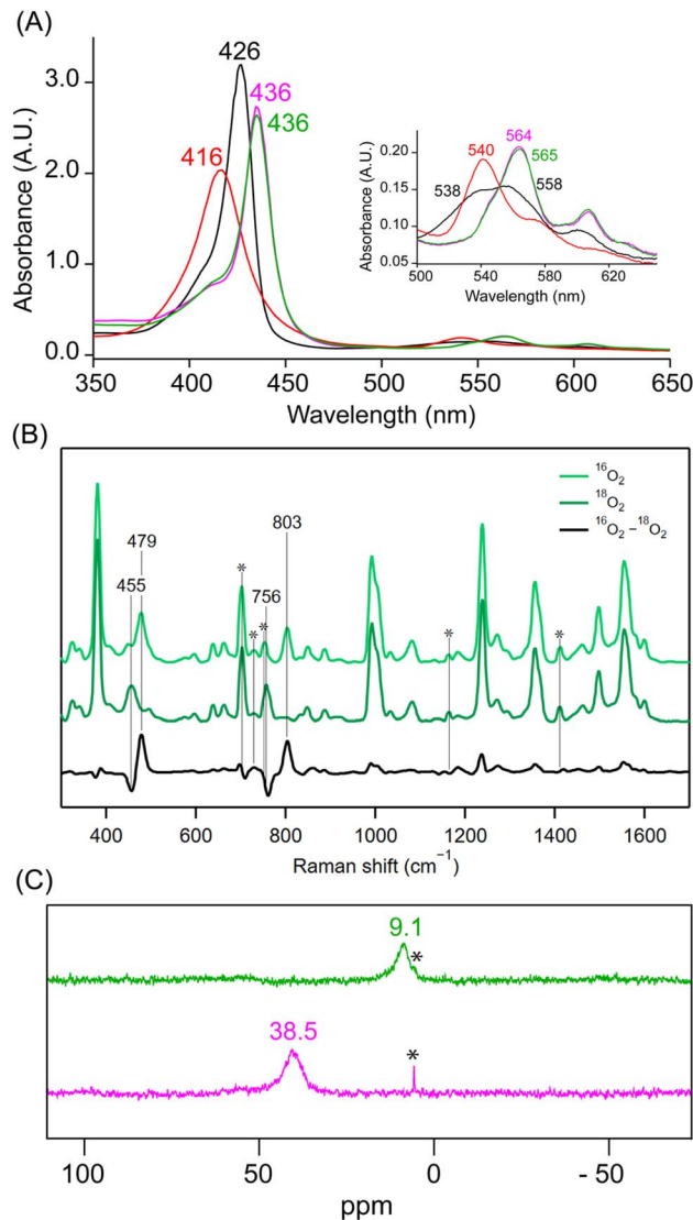
Fig. 2 (A) UV-vis spectra (in 9:1 DCM:THF at -40\text{ }^\circ\text{C} ) for 50 \mu\text{M} solutions of [(THF)_2(TPP)Fe^{II}] (black), [(THF)(TPP)Fe^{III}(O_2^{2-})]^- (red), [(THF)(TPP)Fe^{III}(O_2^{2-})]^- (pink), and [(4\text{-Melm})(TPP)Fe^{III}(O_2^{2-})]^- (green). Inset shows the expanded Q-band region. (B) Resonance Raman spectra ( \lambda_{\text{ex}} = 457\text{ nm} ) collected for a 2 mM 9:1 DCM:THF frozen solution sample of [(4\text{-Melm})(TPP)Fe^{III}(O_2^{2-})]^- prepared with ^{16}\text{O}_2(\text{g}) (light green) and ^{18}\text{O}_2(\text{g}) (dark green); the difference spectrum is shown in black. (C) ^2\text{H} NMR spectra (in 9:1 DCM:THF at -40\text{ }^\circ\text{C} ) for [(THF)(TPP-d_8)Fe^{III}(O_2^{2-})]^- (pink), and [(4\text{-Melm})(TPP-d_8)Fe^{III}(O_2^{2-})]^- (green); *peaks correspond to the solvent.
