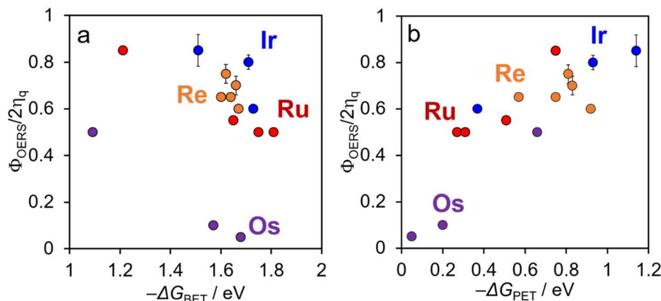
Fig. 8 Plots of \Phi_{\text{OERS}}/2\eta_q for [\text{Re}(\text{PR}_3)_2]^+ (orange), [\text{Ir}(\text{C}^{\wedge}\text{N})_2(\text{N}^{\wedge}\text{N})]^+ (blue), and Ru(II) (red), and Os(II) (purple) tris(diimine) complexes as a function of the driving force for (a) back-electron-transfer between OERSs and \text{BIH}^{++} ( -\Delta G_{\text{BET}} ) and (b) photoinduced electron-transfer ( -\Delta G_{\text{PET}} ).
