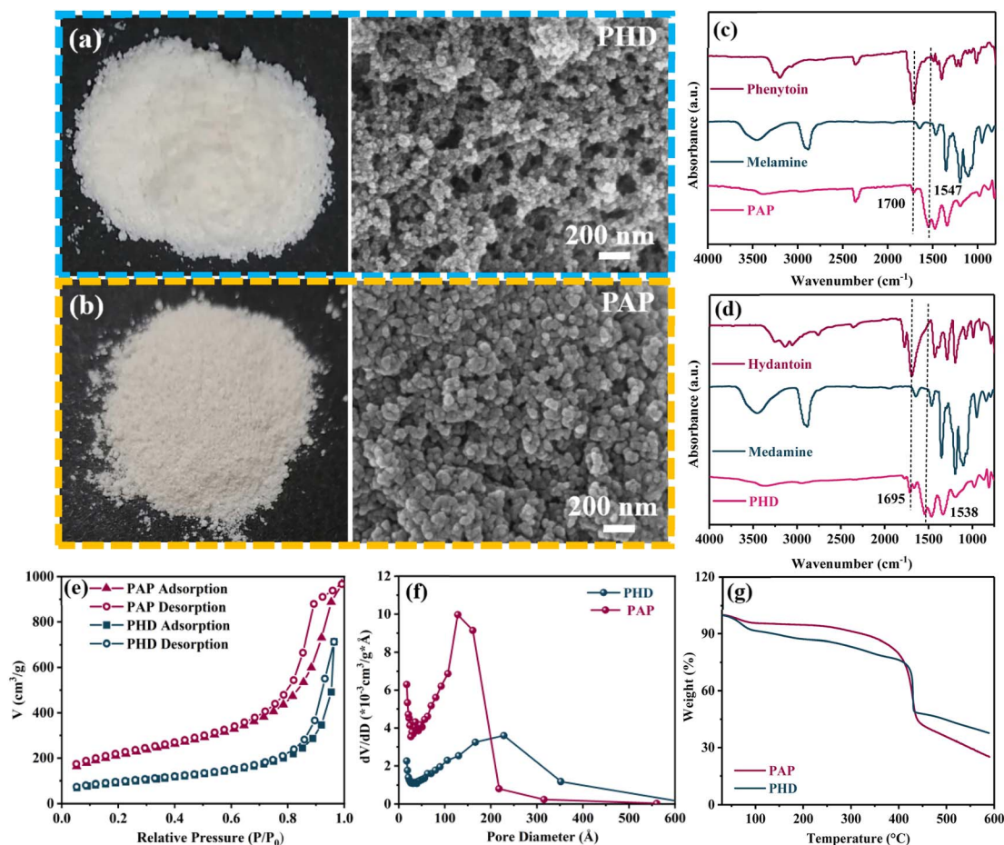
Fig. 2 Photograph and SEM image of (a) PHD and (b) PAP. FTIR spectra in the wavenumber range of 4000–800 cm -1 of (c) PAP and (d) PHD. (e) Nitrogen isotherms at 298 K of PHD and PAP. (f) Pore size distribution of PHD and PAP. (g) TGA curves of PAP and PHD.
