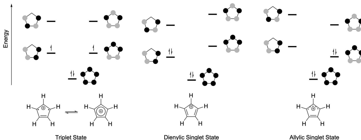
Fig. 1 Structures of the triplet and singlet states of Cp^+ with their \pi -orbital diagrams.
