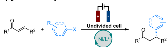
Scheme 1 Design of enantioselective electrochemical reductive conjugate addition.
