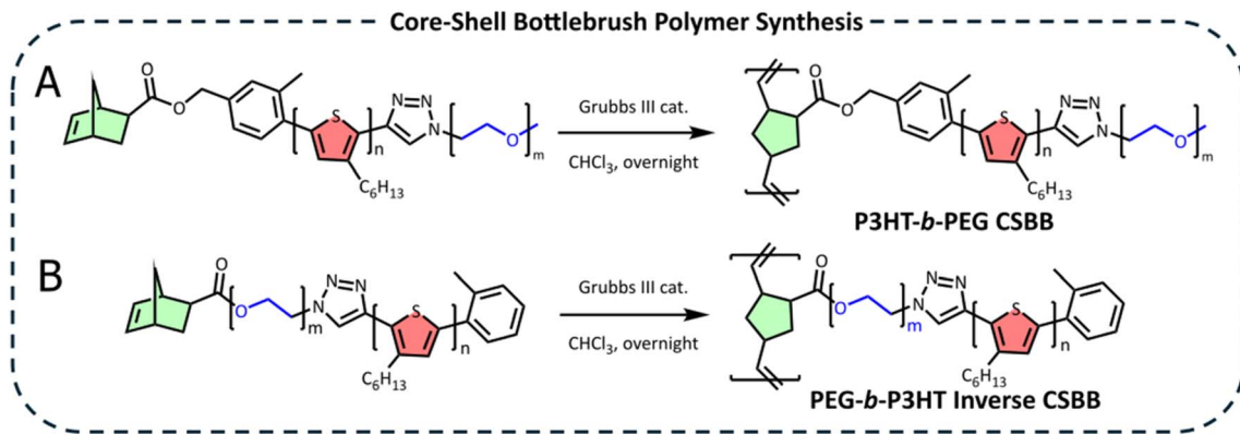
Scheme 2 Ring opening metathesis polymerization of (A) Nor-P3HT- b -PEG and (B) Nor-PEG- b -P3HT using a Grubbs III catalyst to form P3HT- b -PEG CSBB and PEG- b -P3HT ICSBB, respectively.
