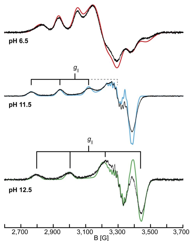
Fig. 2 CW X-band (9.46 GHz) EPR spectra of SmAA10A at pH 6.5, 11.5 and 12.5 in black with EPR simulations in color. The simulation for pH 12.5 uses the 14 N couplings of case A (see section on 14 , 15 N ENDOR). EPR parameters are listed in Tables 1 and S1† and experimental conditions are reported in the Experimental section.
