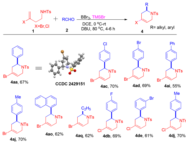
Scheme 3 Synthesis of 4-halo-1,2,3,6-tetrahydropyridines. a Reaction conditions: 1 (0.6 mmol), 2 (0.66 mmol), \text{BBr}_3 (0.15 mmol), \text{TMSBr} (0.72 mmol), DCE (3 mL), 0\text{ }^\circ\text{C} -rt, DBU (24.0 mmol), \text{N}_2 atmosphere.
