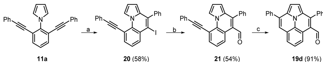
Scheme 5 Selective synthesis of 19d . Conditions: (a) I_2 , NaHCO_3 , DCM, 0\text{ }^\circ\text{C} ; (b) t\text{-BuLi} , THF, -78\text{ }^\circ\text{C} , then dry DMF, -78\text{ }^\circ\text{C} then r.t.; (c) InCl_3 , toluene, reflux.
