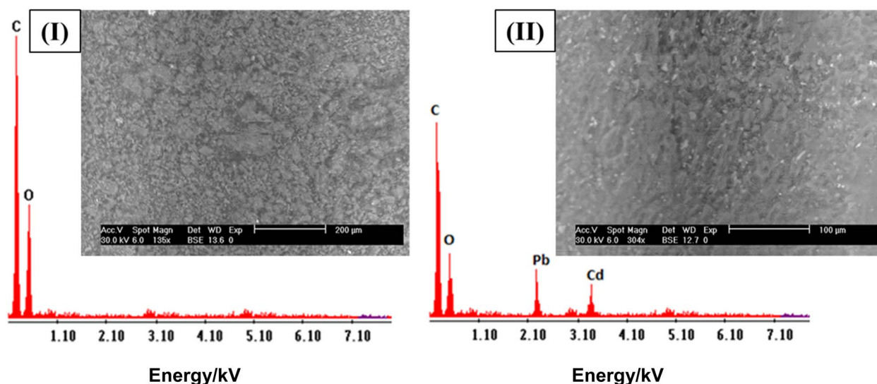
Fig. 8 SEM images and EDX spectrum of the ligand before (I) and after (II) sorption.
