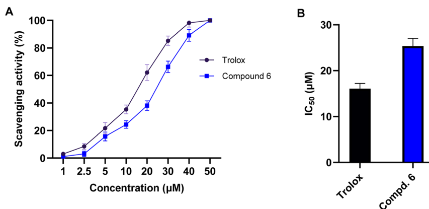
Fig. 7 The free radical scavenging activity of compound 6 toward DPPH radicals. (A) The dose-dependent scavenging activity of compound 6 and Trolox standard toward DPPH radicals. The presented data is displayed in triplicate as mean \pm SD. (B) Representation of the \text{IC}_{50} values of compound 6 and Trolox toward DPPH radicals.
