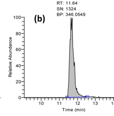
Fig. 1 Comparison of representative chromatographic peaks of the standards covering various chemical classes analyzed with LC-MS using (a) Z-HILIC and (b) ZIC-pHILIC columns. The peak quality of all standards was assessed and compared for both methods as illustrated in Fig. 2.
