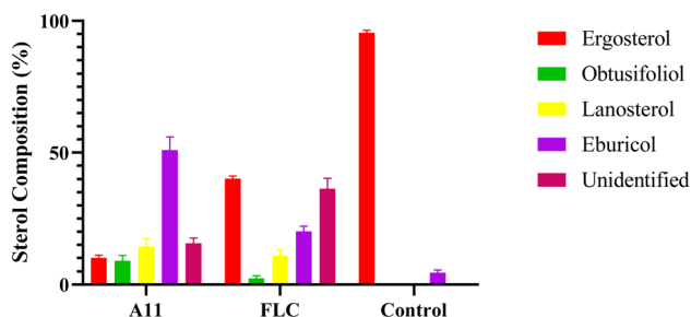
Fig. 3 Sterol composition analysis. FLC and A11 were co-cultured with C. alb SC5314 for 24 h at 0.03 μg mL -1 . Bars represent the mean ± SD ( n = 3).
