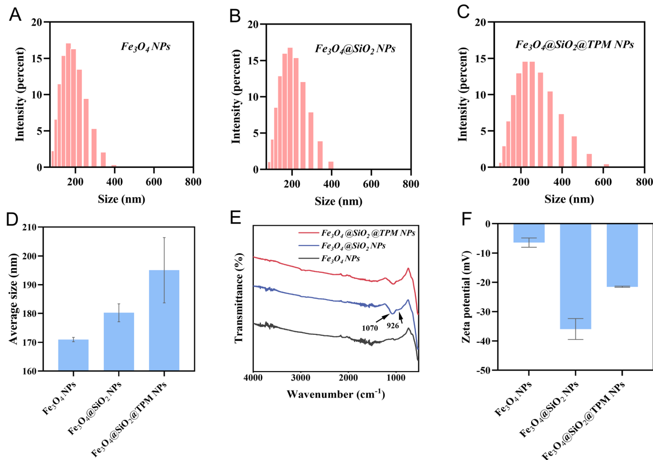
Fig. 2 Characterization of the double-bond functionalized \text{Fe}_3\text{O}_4 NPs. Particle size distribution of (A) \text{Fe}_3\text{O}_4 NPs, (B) \text{Fe}_3\text{O}_4@\text{SiO}_2 NPs, and (C) \text{Fe}_3\text{O}_4@\text{SiO}_2@\text{TPM} NPs. (D) Average particle size analysis, (E) FTIR spectra, and (F) zeta potentials of \text{Fe}_3\text{O}_4 , \text{Fe}_3\text{O}_4@\text{SiO}_2 , and \text{Fe}_3\text{O}_4@\text{SiO}_2@\text{TPM} NPs. From \text{Fe}_3\text{O}_4 to \text{Fe}_3\text{O}_4@\text{SiO}_2@\text{TPM} NPs, their particle size distributions increased, and their average particle sizes expanded. In comparison with the FTIR spectrum of \text{Fe}_3\text{O}_4 , \text{Fe}_3\text{O}_4@\text{SiO}_2 NPs appeared two new peaks at 1070 and 926 \text{cm}^{-1} , ascribing to the Si–O–Si stretching vibrations, and the Si–OH stretching vibration. In comparison with the FTIR spectrum of \text{Fe}_3\text{O}_4@\text{SiO}_2 NPs, \text{Fe}_3\text{O}_4@\text{SiO}_2@\text{TPM} NPs observed two peaks at 2960 and 2920 \text{cm}^{-1} corresponding to the symmetric C–H stretches of methyl (– \text{CH}_3 ) groups. In comparison with the zeta potential of \text{Fe}_3\text{O}_4 , \text{Fe}_3\text{O}_4@\text{SiO}_2 NPs decreased to -36.71 \pm 3.30 mV due to the presence of Si–OH groups on their surface. The zeta potential of \text{Fe}_3\text{O}_4@\text{SiO}_2@\text{TPM} NPs increased to -21.52 \pm 0.21 mV because of the reduction in Si–OH groups and the increase in double bonds.
