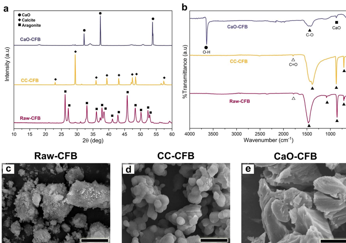
Fig. 2 (a) XRD patterns and (b) FTIR spectra of the raw-CFB, CC-CFB, and CaO-CFB. (c–e) Morphologies of the raw-CFB, CC-CFB, and CaO-CFB. Scale bars: 5 \mu\text{m} (c–e).
