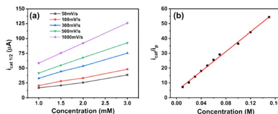
Fig. 6 Plot of i_{\text{cat}1/2} (half-way catalytic current) in the function of the concentration of NiL complex at different potential scan rates in the presence of 70 \text{ mM} acetic acid as the proton source (a). A plot of i_{\text{cat}1/2}/i_p as a function of acetic acid concentration while using 1 \text{ mM} NiL , the potential scan rate of 50 \text{ mV s}^{-1} (b).
