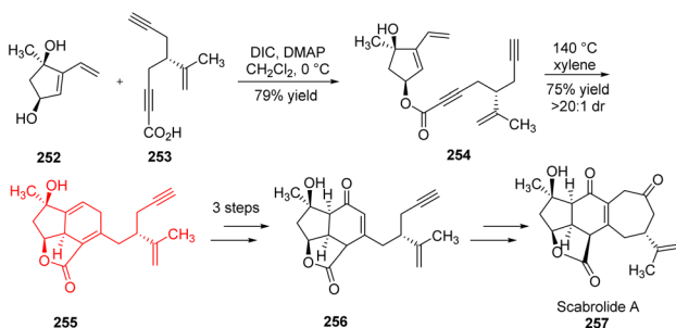
Scheme 32 Total synthesis of scabrolide A ( 257 ). 78
