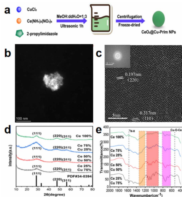
Fig. 1 Preparation and characterization of CeO 2 @Cu-PrIm. (a) Schematic depicting the synthesis process. (b) TEM image of CeO 2 @Cu-PrIm. (c) HRTEM image of CeO 2 @Cu-PrIm. (d) XRD pattern. (e) FT-IR spectral analysis. (d) and (e) Contained samples synthesized using different copper and cerium metal ion doping ratios and the grey line represented CeO 2 @Cu-PrIm.
