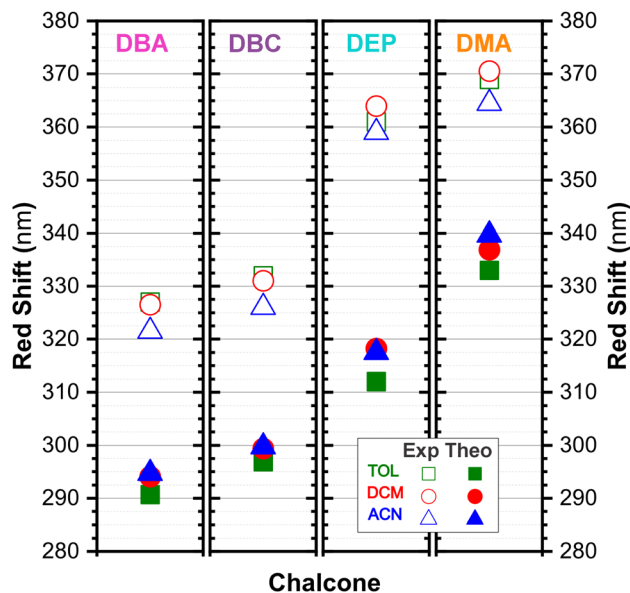
Fig. 11 Dibenzoalacetone derivatives experimental red-shift in TOL (open green squares), DCM (open red circles), and ACN (open blue triangles) with theoretical red-shift, using the TD-DFT methodology and M06-2X functional, and the 6-311+G(d,p) basis set with the implicit solvent method (IEFPCM) in TOL (solid green squares, \kappa_{\text{TOL}} = 2.37 ), DCM (solid red circles, \kappa_{\text{DCM}} = 8.93 ) and ACN (solid blue triangles, \kappa_{\text{ACN}} = 35.67 ).
