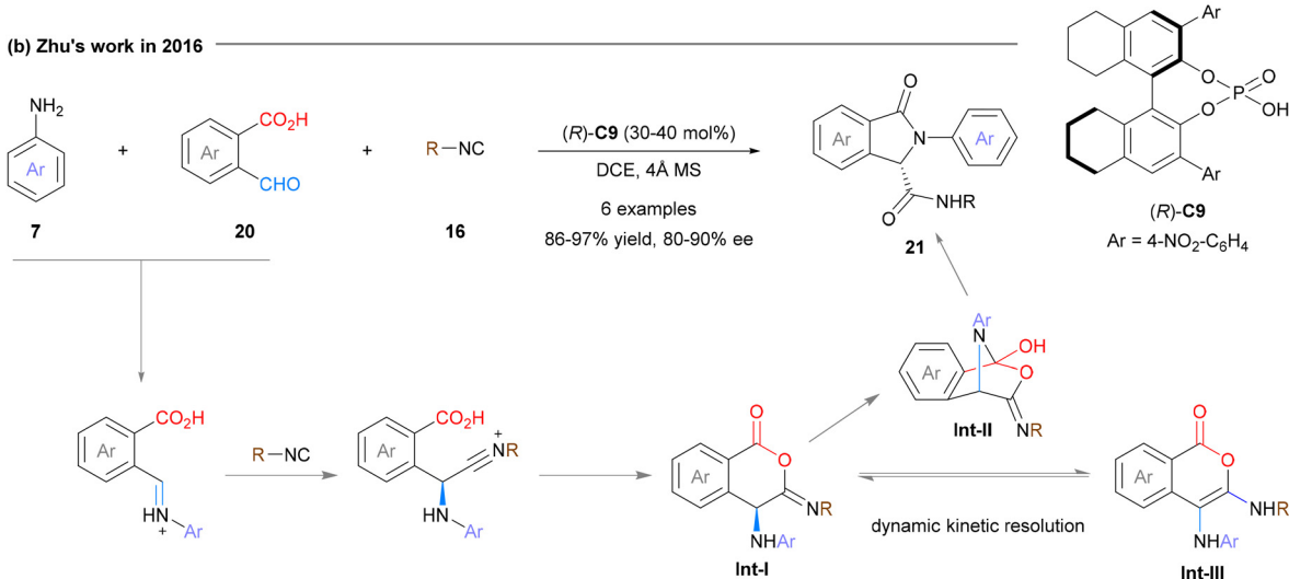
Fig. 5 Initial attempts on enantioselective Ugi-type three-component reactions.
