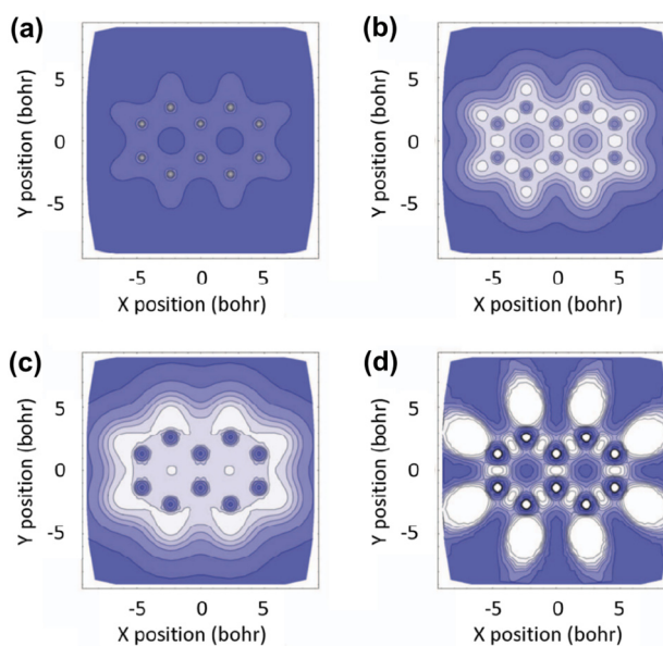
Fig. 34 EDR and ELF plots for the naphthalene molecule, computed at the DFT level (PBE0/6-311G(2d,2p)). (a) EDR plot calculated at the delocalization length of u = 0.25 bohr shows the core electrons. (b) EDR at u = 1 bohr represents the delocalization of the electrons forming single bonds. (c) The electron delocalization over the aromatic rings becomes apparent at EDR obtained for the bigger u = 2 bohr. (d) Plot of the electron localization function (ELF). Reprinted with permission from the original paper by Janesko and co-workers. 17
