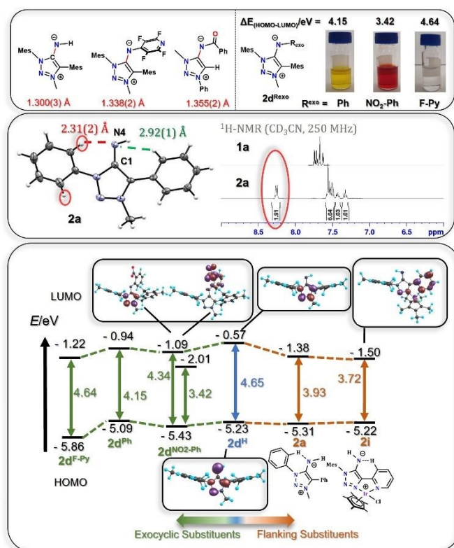
Figure 1 Top: C1-N4 bond lengths and the colours of MIIs with different R^{\text{exo}} substituents. Middle: Intramolecular H-bonds are highlighted in solid state and in solution. Bottom: MO-diagram with the frontier orbitals (HOMO, LUMO and LUMO +1) and the corresponding energy levels for differently substituted MIIs. The localised Kohn-Sham orbitals are displayed only for selected compounds to remain clarity of the figure. Level-of-theory: PBE0/def2-TZVP/SARC-ZORA-TZVP(Ir)/CPCM( \text{CH}_2\text{Cl}_2 ) 84-87 .
