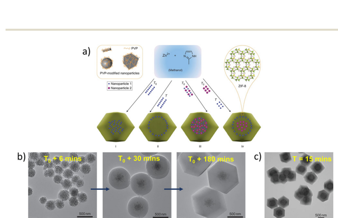
Fig. 13 (a) A diagram showing how the addition sequence of the PVP-modified nanoparticles during MOF synthesis played a role in the spatial distribution of the incorporated PVP-modified nanoparticles within the ZIF-8 crystals at T_0 or T during the MOF synthesis, (b) TEM images of the intermediate products of Au nanoparticle/ZIF-8 hybrid crystals collected at different reaction times: 6 minutes, 30 minutes, and 180 minutes after nanoparticle addition, (c) TEM image of hybrid crystals obtained when Au nanoparticles AuNPs were added 15 minutes after the initiation of the reaction. Adapted with permission from ref. 57. Copyright 2012 Springer Nature.
