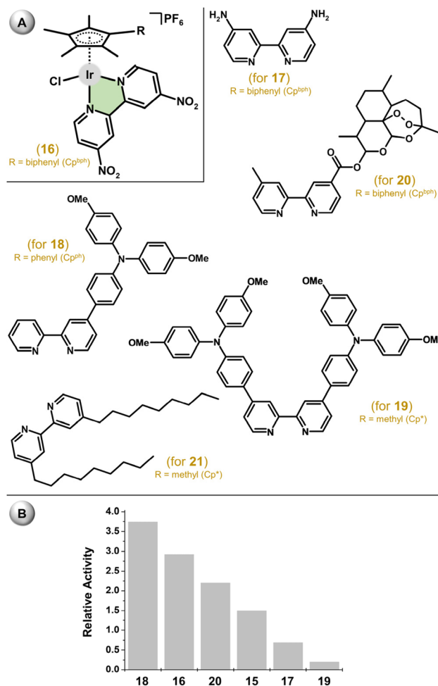
Fig. 6 (A) The structural formula of complex 16 and bpy-based ligands of analogues 17 – 21 , and (B) comparison of the in vitro antiproliferative activity of 15 – 20 against the A549 lung carcinoma cell line (given as relative activity). Complex 15 (see Fig. 5) is given for comparative purposes. Complex 21 was not tested in A549 cells.
