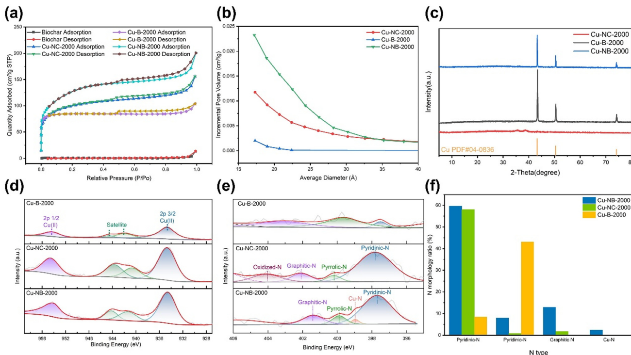
Fig. 2 (a) N 2 adsorption and desorption isotherms of fecal-derived biochar, Cu-NB-2000, Cu-NC-2000 and Cu-B-2000. (b) The incremental pore volume of Cu-NC-2000, Cu-B-2000, and Cu-NB-2000. (c) XRD patterns of Cu-NC-2000, Cu-B-2000 and Cu-NB-2000. The high-resolution (d) Cu 2p and (e) N 1s XPS spectra of Cu-B-2000, Cu-NC-2000 and Cu-NB-2000. (f) The proportion of different N types for Cu-NB-2000, Cu-NC-2000, and Cu-B-2000 catalysts.
