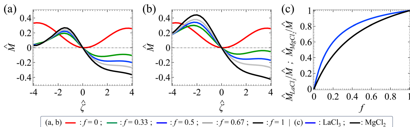
Fig. 5 (a) The non-dimensionalized diffusiohoretic mobility \hat{M} versus the non-dimensionalized colloid surface potential \hat{\zeta} in the same porous media (the ratio of the screening length to the colloid radius l/a = 0.75 ) saturated with solution mixtures of p molar of KCl and q molar of LaCl 3 with different compositions f = q/(p + q) . The solution ionic strength I = 1 mM. Red line: f = 0 . Green line: f = 0.33 . Blue line: f = 0.5 . Grey line: f = 0.67 . Black line: f = 1 . (b) \hat{M} versus \hat{\zeta} in the same porous media ( l/a = 0.75 ) saturated with solution mixtures of p molar of KCl and q molar of MgCl 2 with different compositions f = q/(p + q) . The color scheme and the ionic strength are the same as (a). (c) The ratio of the contribution to the mobility by the asymmetric electrolyte to that by the mixture \hat{M}_{\text{LaCl}_3}/\hat{M} and \hat{M}_{\text{MgCl}_2}/\hat{M} versus f . Blue line: \hat{M}_{\text{LaCl}_3}/\hat{M} . Black line: \hat{M}_{\text{MgCl}_2}/\hat{M} .
