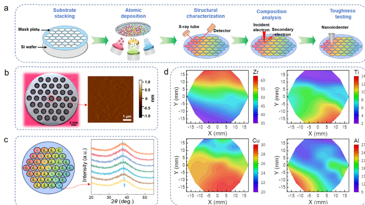
Fig. 1 (a) A schematic diagram of high-throughput development strategy of tough MGFs. (b) The optical picture of the fabricated Zr–Ti–Cu–Al MGF material library and the surface morphology of one marked subregion by AFM. The red dashed circle marks the selected subregion. (c) XRD patterns for 37 subregions within Zr–Ti–Cu–Al MGF material library. The right plot gives the detailed XRD patterns corresponding to the 7 selected subregions along the blue dashed line. (d) The distribution diagrams of the elements of Zr, Cu, Ti and Al in the fabricated Zr–Ti–Cu–Al MGF material library.
