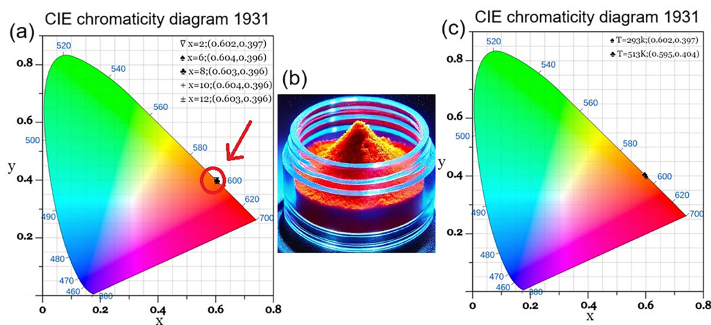
Fig. 13 (a) Chromaticity coordinates of \text{Ca}_3\text{La}_7(\text{SiO}_4)_5(\text{PO}_4)\text{O}_2:x \text{ at } \% \text{Sm}^{3+} ( x = 2, 6, 8, 10 and 12 ); (b) a photograph of the orange-red \text{Ca}_3\text{La}_7(\text{SiO}_4)_5(\text{PO}_4)\text{O}_2:6 \text{ at } \% \text{Sm}^{3+} phosphor under blue light illuminant at room temperature; (c) chromaticity coordinates of \text{Ca}_3\text{La}_7(\text{SiO}_4)_5(\text{PO}_4)\text{O}_2:6 \text{ at } \% \text{Sm}^{3+} phosphors (at 293 K and 513 K) in the CIE 1931 chromaticity diagram.
