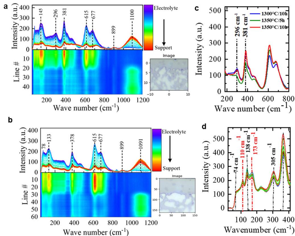
Fig. 7 Line averaged Raman spectra obtained from mapped areas of polished cross-sections of (a) BSZCY44362|NiO-BSZCY541 half-cell sintered at 1300 °C for 10 hours. (b) Polished cross-section of the half-cell sintered at 1350 °C for 5 hours the optical images. (c) Raman spectra from the electrolyte layer only, highlighting the well-resolved Y-O mode at 296 cm -1 . (d) Raman spectra from the polished cross-section of the half-cell sintered at 1400 °C.
