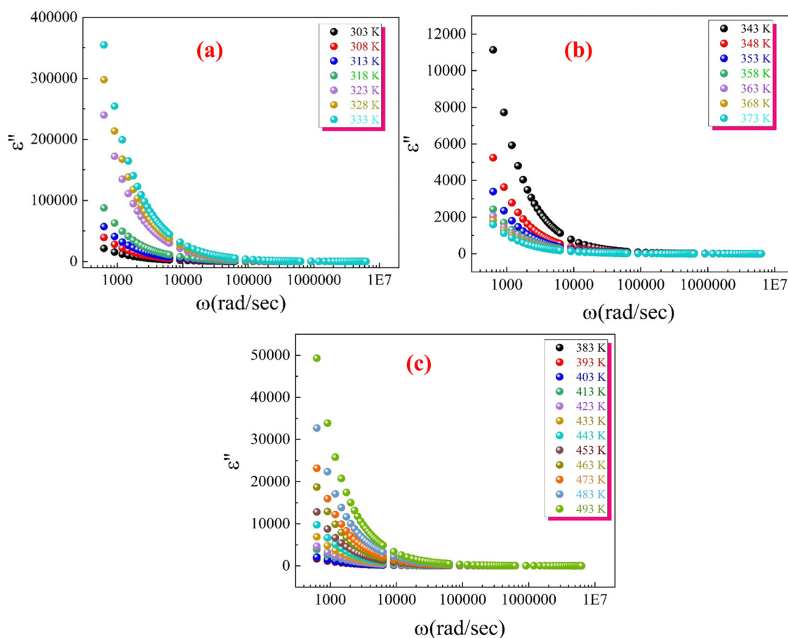
Fig. 23 Variation of the imaginary part of the permittivity \varepsilon'' with the angular frequencies (a) for the first temperature region (303–333 K), (b) for the second temperature region (343–373 K), and (c) for the third temperature region (383–493 K) for the synthesized CFO ferrite nanoparticles.
