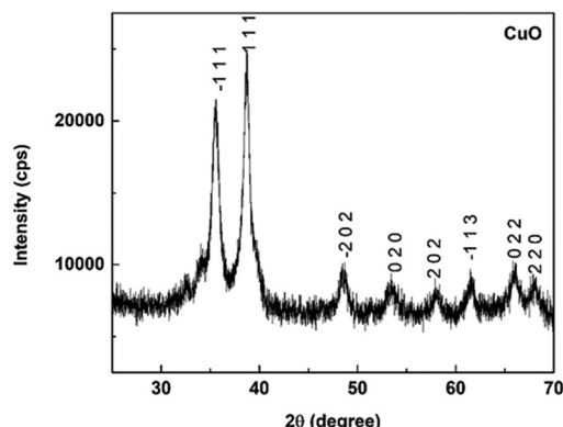
Fig. 3 Graphical representation of the XRD pattern of CuO NPs.
