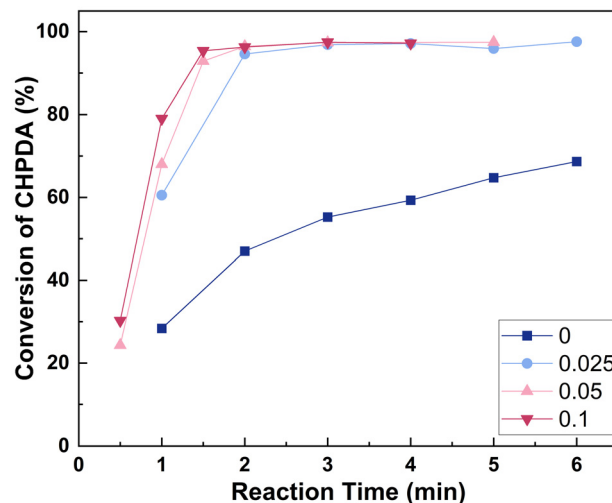
Fig. 9 Effect of n(\text{TBACl})/n(\text{CHPDA}) on the reaction. Reaction conditions: n(\text{NaOH}) : n(\text{CHPDA}) = 1.05 : 1 and T = 100\text{ °C} , and the concentrations of the TBACl and NaOH solutions are 20 wt%.
